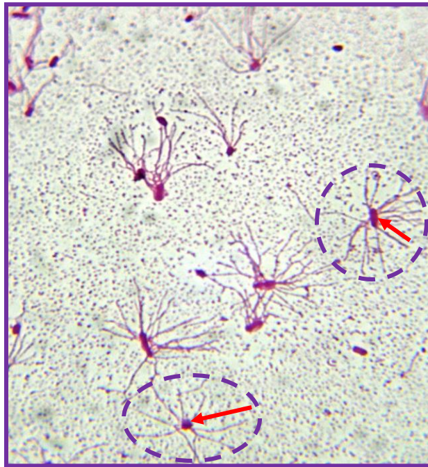
peritrichous arrangement
